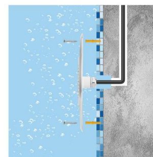
2D Installation Diagram
