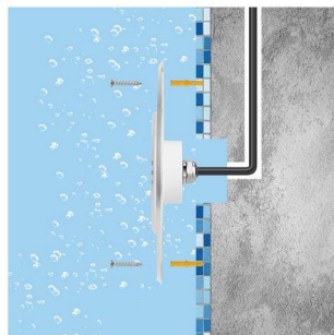
2D Installation Diagram
