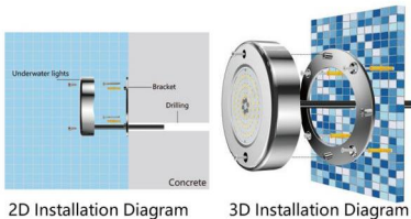
2D Installation Diagram 3D Installation Diagram
