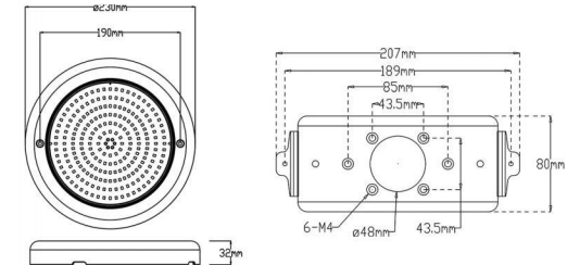
SS-JPB230-18W / SS-JPB230-25W SS-JPB230-35W / SS-JPB230-42W Optional Accessories Mounting Bracket(SS316L)
