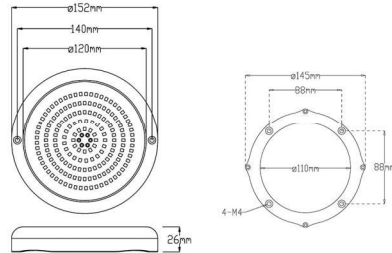
SS-JPB152-10W SS-JPB152-18W Optional Accessories Mounting Bracket(SS316L)
