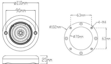
SS-JPB110-6W Optional Accessories Mounting Bracket(SS316L)
