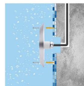
2D Installation Diagram
