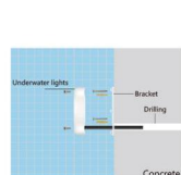
2D Installation Diagram
