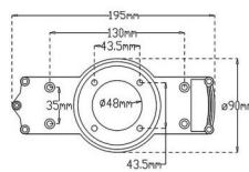
Optional Accessories Mounting Bracket(ABS)
